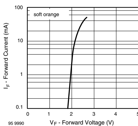
Fig. 10 - Forward Current vs. Forward Voltage
