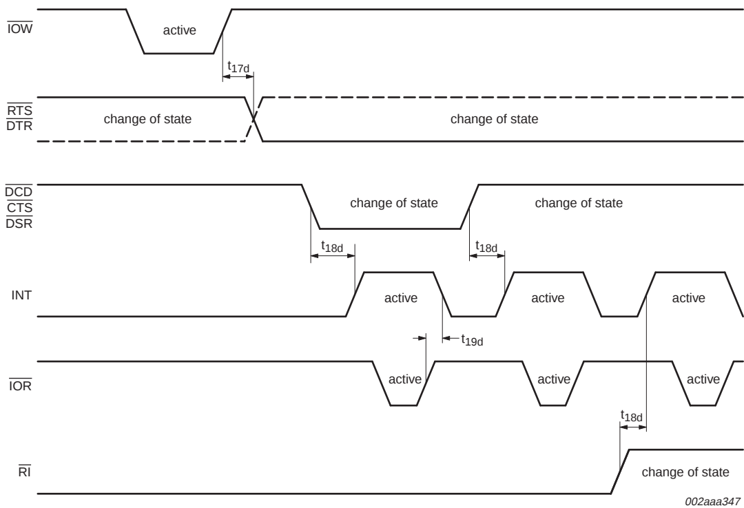
Fig 16. Modem input/output timing
