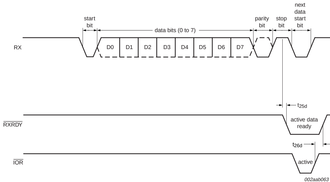
Fig 19. Receive ready timing in non-FIFO mode
