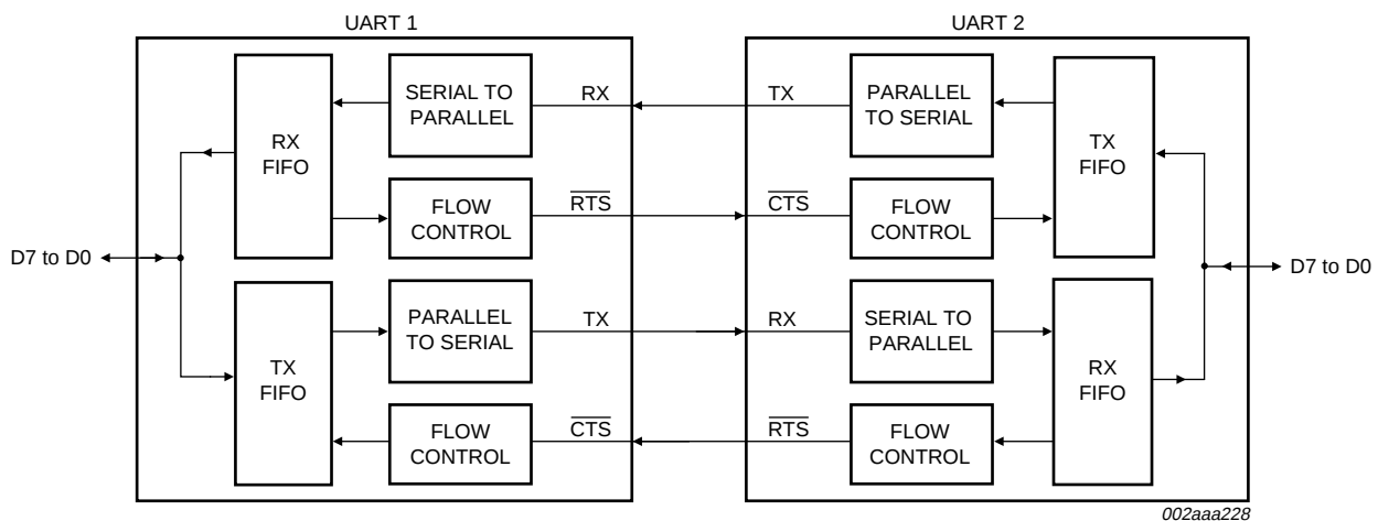
Fig 6. Autoflow control (auto- \overline{\text{RTS}} and auto- \overline{\text{CTS}} ) example
