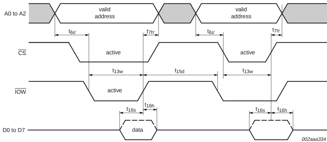
Fig 15. General write timing when \overline{AS} is tied to V_{SS}
