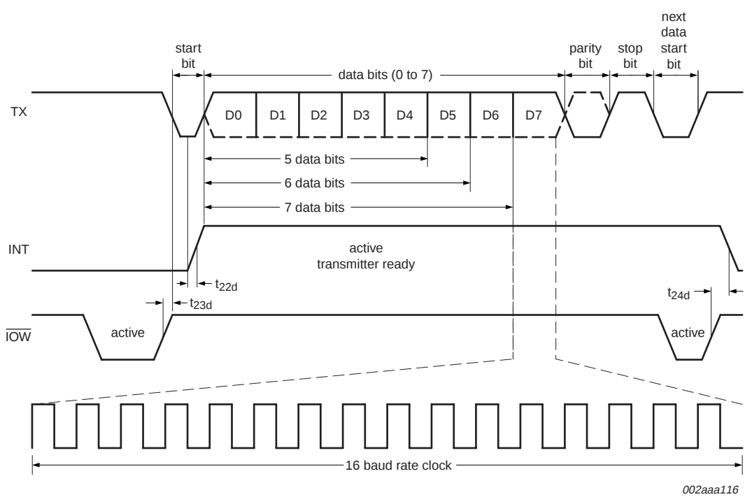
Fig 21. Transmit timing
