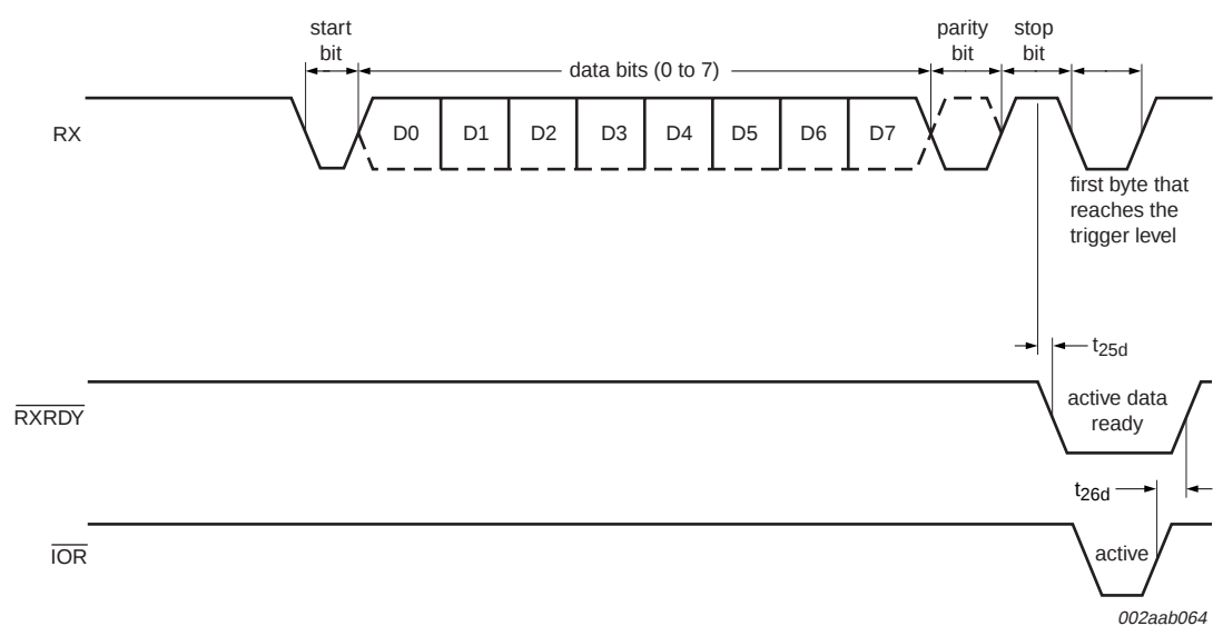
Fig 20. Receive ready timing in FIFO mode
