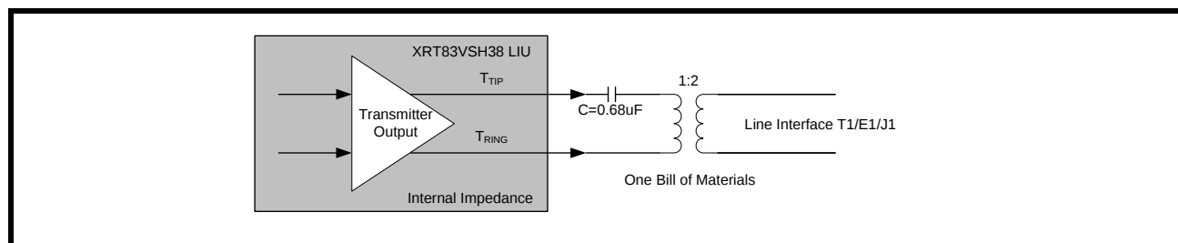
FIGURE 21. TYPICAL CONNECTION DIAGRAM USING INTERNAL TERMINATION
