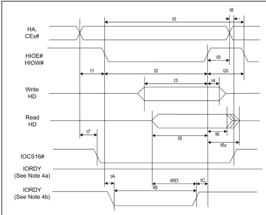
Figure 9 Read/Write Timing Diagram, PIO Mode
