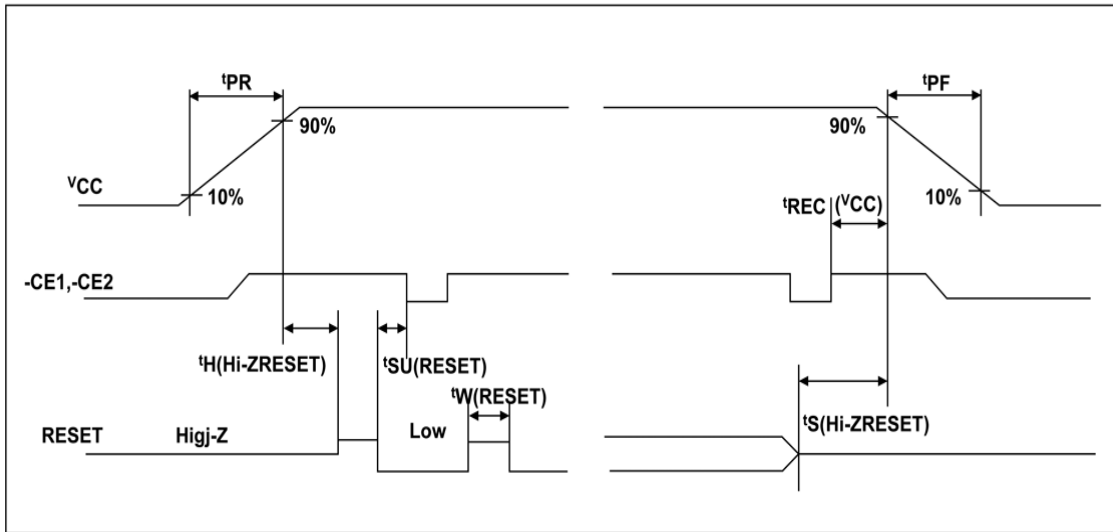
Figure 15 Timing Diagram, Hardware Reset
