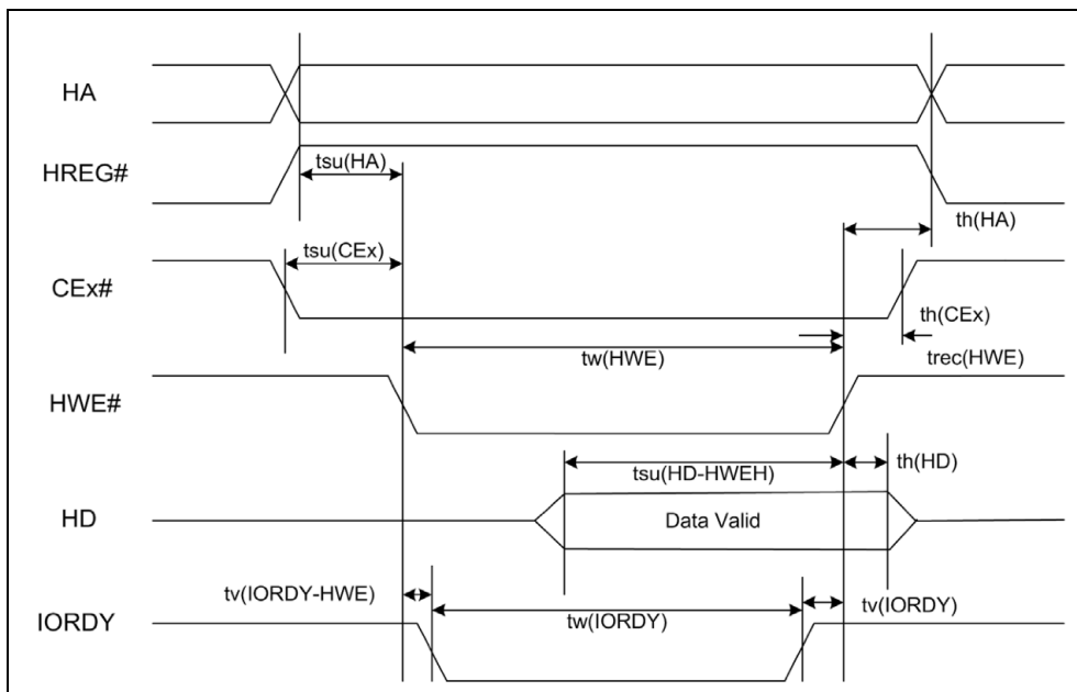
Figure 6 Common Memory Write Timing Diagram
