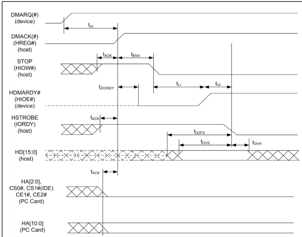
Figure 12 Ultra DMA Mode Data-out Burst Initiation Timing Diagram
