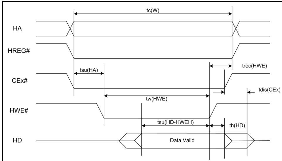
Figure 4 Configuration Register (Attribute Memory) Write Timing Diagram
