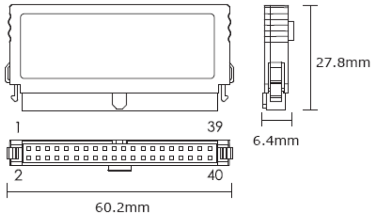
Figure 1 Mechanical Dimension of InnoLite EDC 40pin
