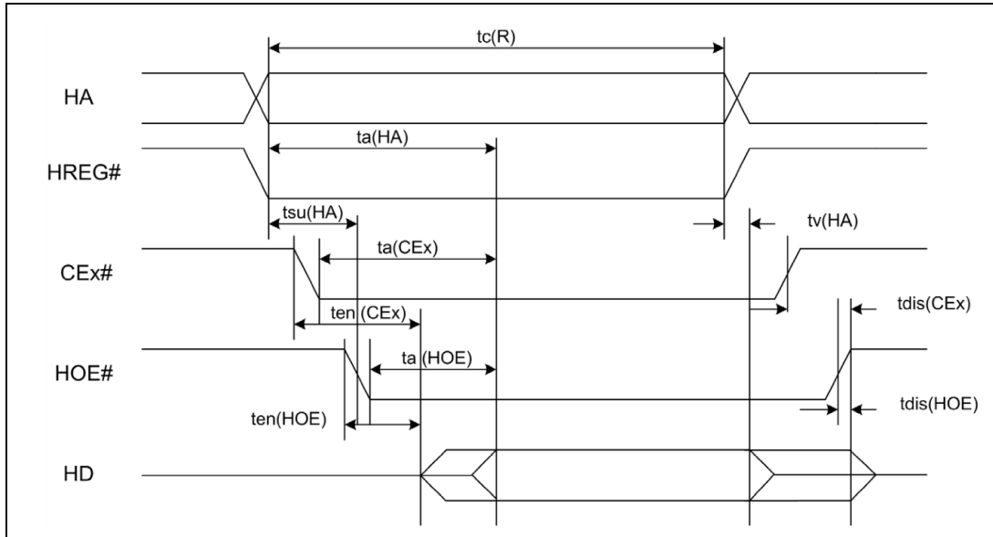
Figure 3: Attribute Memory Read Timing Diagram
