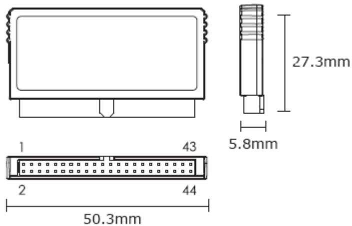
Figure 2 Mechanical Dimension of InnoLite EDC 44pin
