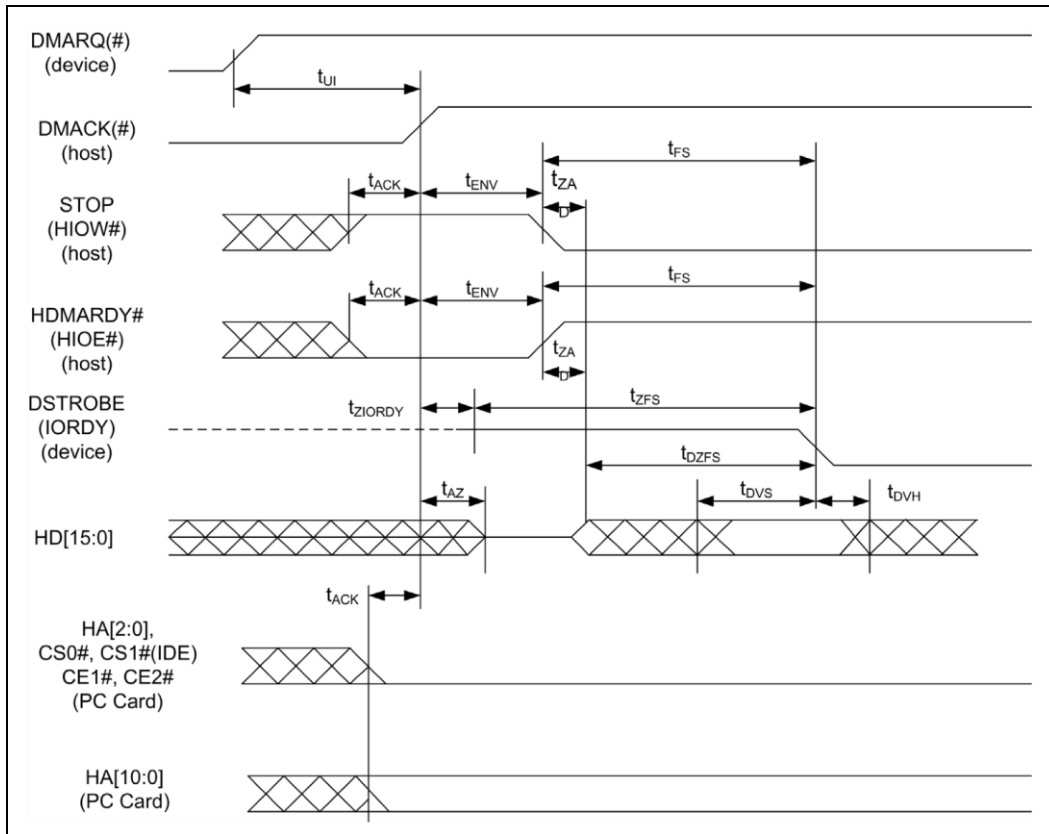
Figure 11 Ultra DMA Mode Data-in Burst Initiation Timing Diagram
