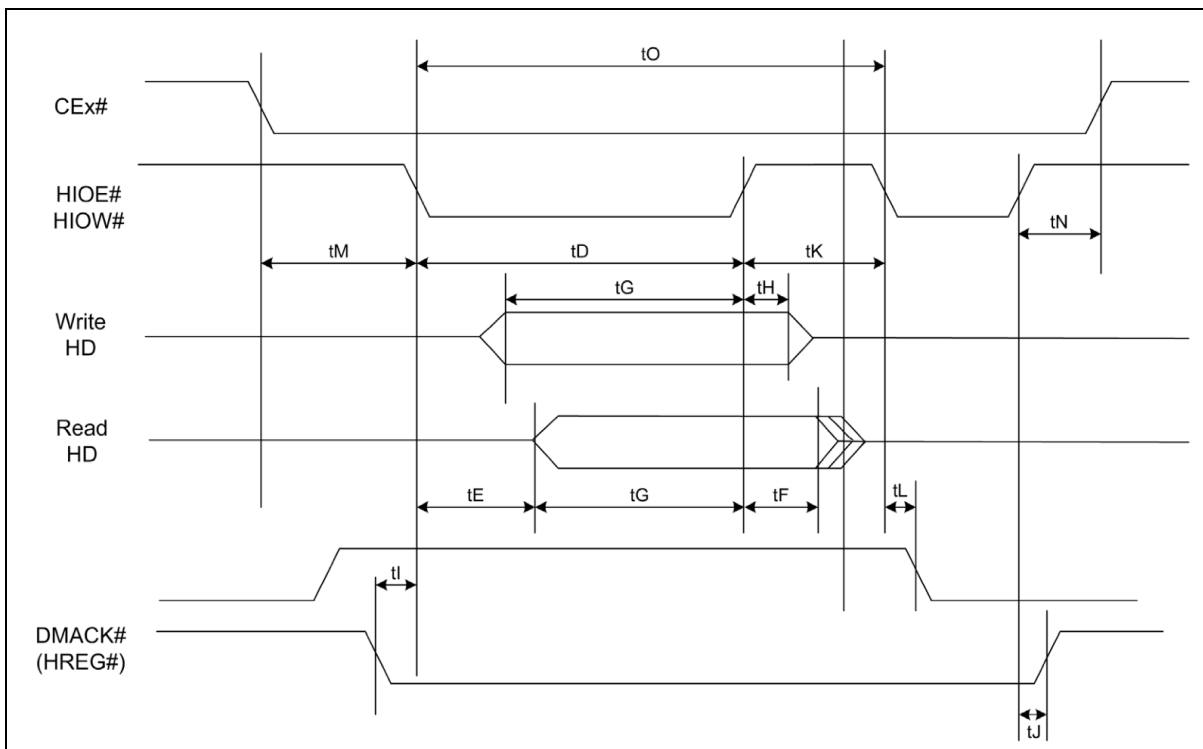
Figure 10 Read/Write Timing Diagram, Multiword DMA Mode
