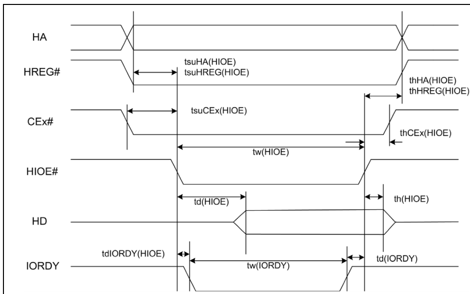
Figure 7 I/O Read Timing Diagram
