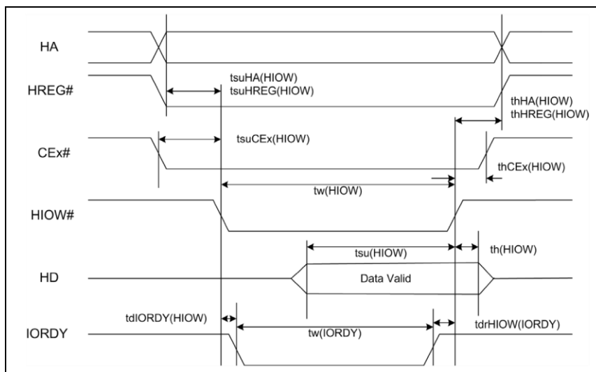
Figure 8 I/O Write Timing Diagram
