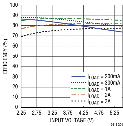
Efficiency vs Input Voltage V_{TT} = 0.9\text{V}
