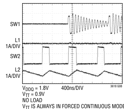
Pulse-Skipping Mode
