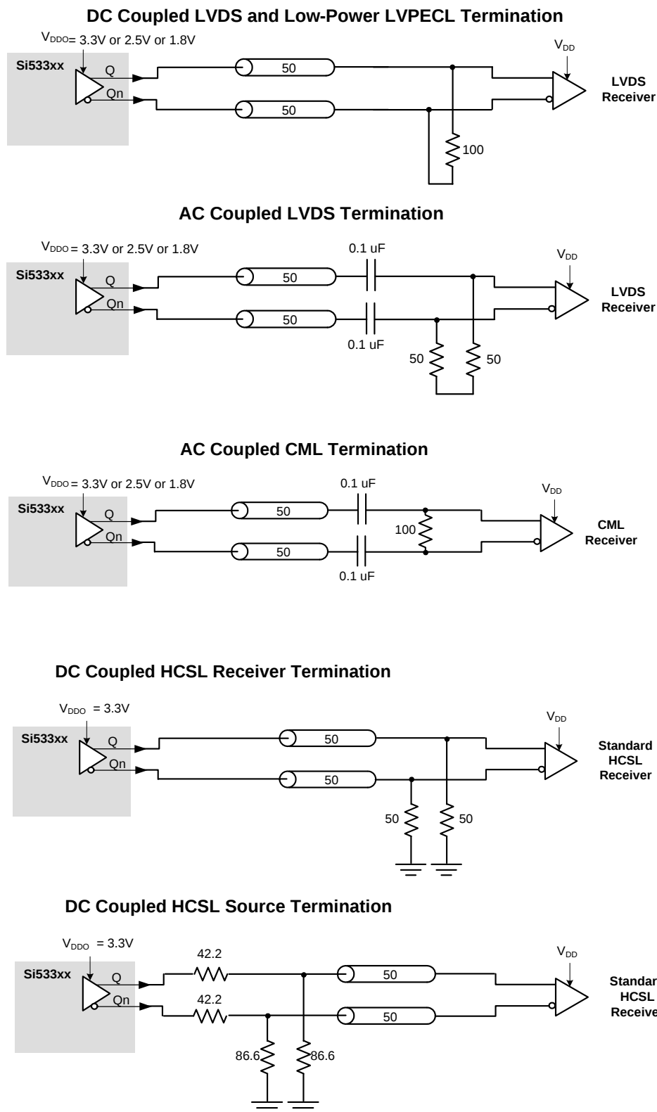
Figure 8. LVDS, CML, and HCSL Output Termination
