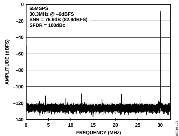
Figure 26. AD9650-65 Single-Tone FFT with f_{IN} = 30.3 MHz at -6 dBFS with Dither Enabled
