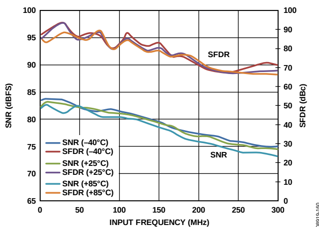
Figure 57. AD9650-105 Single-Tone SNR/SFDR vs. Input Frequency ( f_{IN} )
