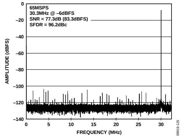
Figure 25. AD9650-65 Single-Tone FFT with f_{IN} = 30.3 MHz at -6 dBFS with Dither Disabled
