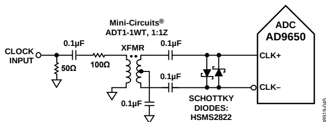
Figure 87. Transformer-Coupled Differential Clock (Up to 200 MHz)
