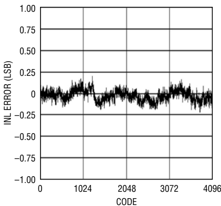
LTC2291: Typical INL, 2V Range, 25Mpsps
