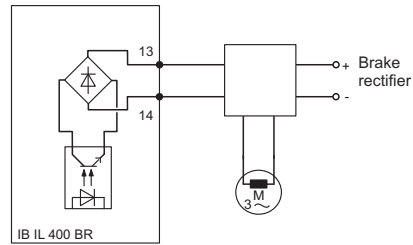
Connection diagram
