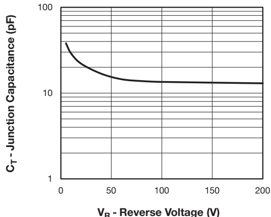
Fig. 3 - Typical Junction Capacitance vs. Reverse Voltage
