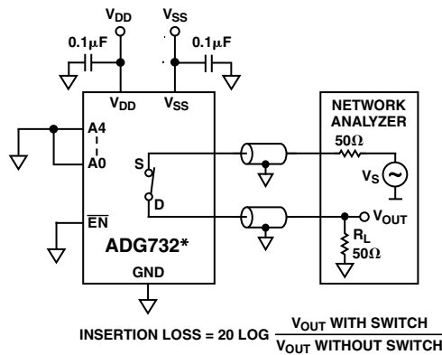
Test Circuit 12. Bandwidth
