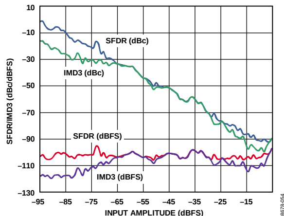
Figure 9. Two-Tone SFDR/IMD3 vs. Input Amplitude (AIN) with f_{IN1} = 28.3 MHz and f_{IN2} = 30.6 MHz
