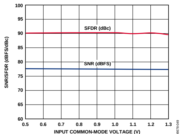
Figure 36. SNR/SFDR vs. Input Common-Mode Voltage, f_{IN} = 32.5 \text{ MHz} , f_s = 80 \text{ MSPS}
