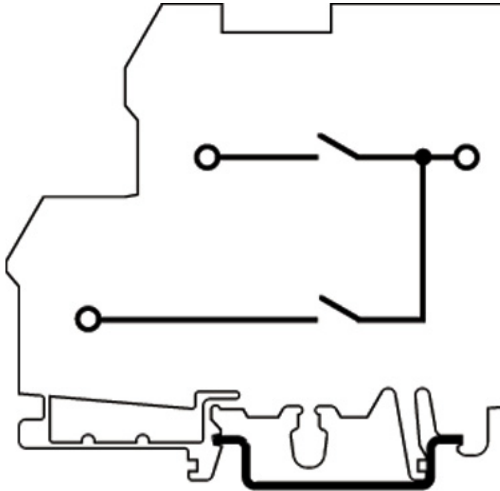
Circuit diagram
