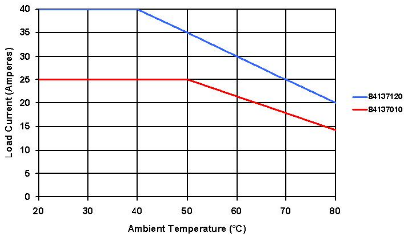
HS151DR w/25 or 50A SSR
