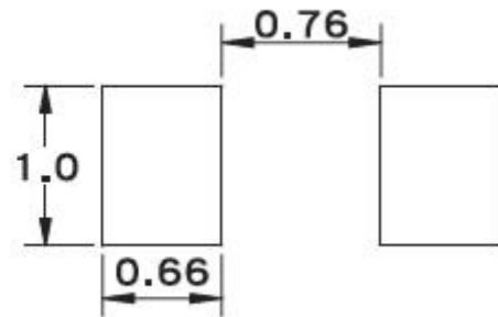
Reflow Solder
