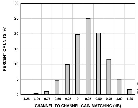
Figure 23. Gain Match Histogram for V_{\text{GAIN}} = 0.8 \text{ V}
