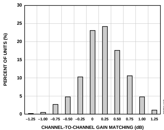
Figure 22. Gain Match Histogram for V_{\text{GAIN}} = 0.2 \text{ V}
