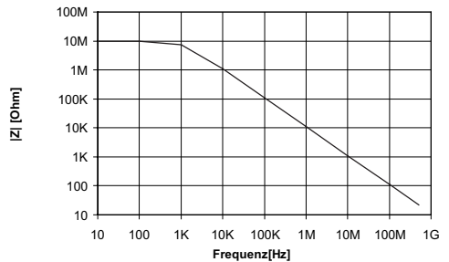
Typical input impedance PMTG311A-RO
