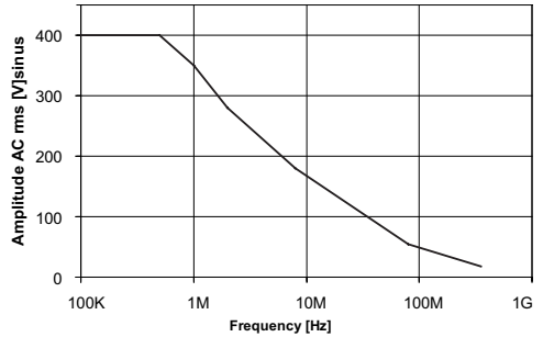
Typical voltage derating PMTG311A-RO Measurement category I
