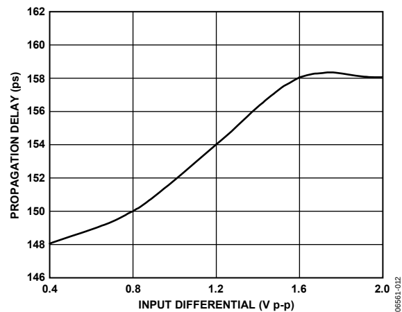
Figure 12. Propagation Delay vs. V_{ID} ; V_{ICM} = 2.15 V
