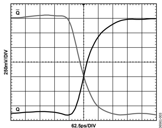
Figure 3. Output Waveform at 1 GHz, V_{CC} = 3.3\text{ V}
