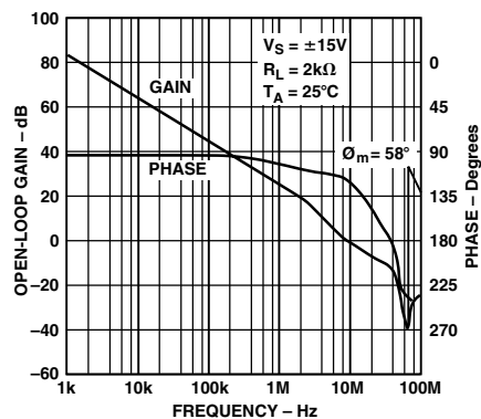
TPC 9. Open-Loop Gain, Phase vs. Frequency
