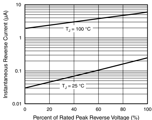
Figure 5. Typical Reverse Leakage Characteristics Per Diode
