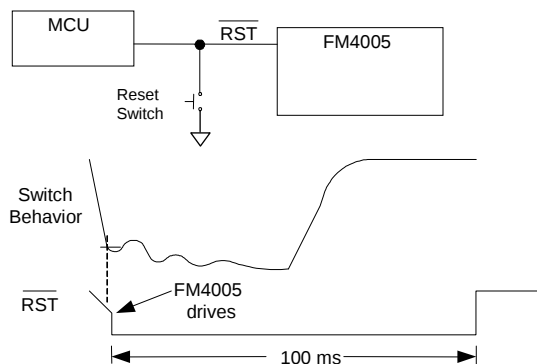
Figure 4. Manual Reset
