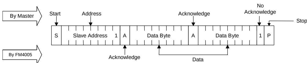
Figure 13. Multiple Register Read
