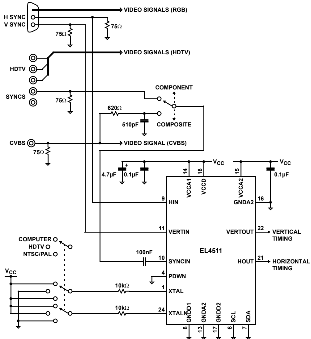
FIGURE 9. APPLICATIONS DRAWING 2
