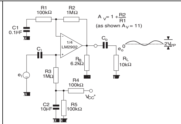
Figure 19. AC coupled non-inverting amplifier
