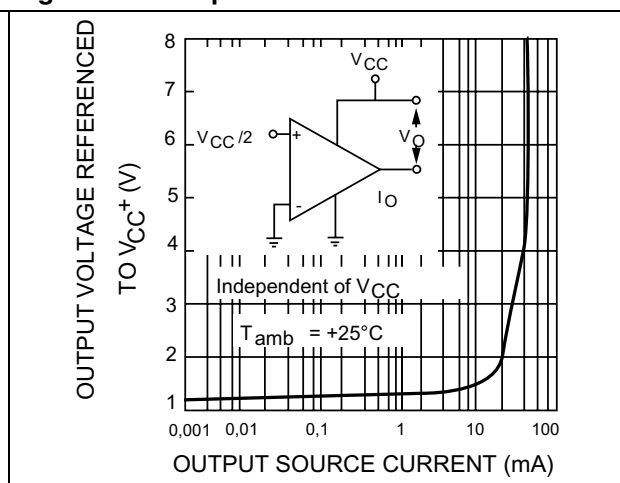
Figure 13. Output characteristics
