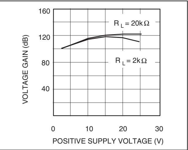
Figure 15. Voltage gain
