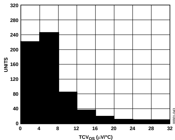
Figure 43. OP482 TCV OS Distribution P Package
