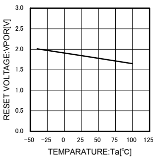
Fig.15 Reset release voltage
