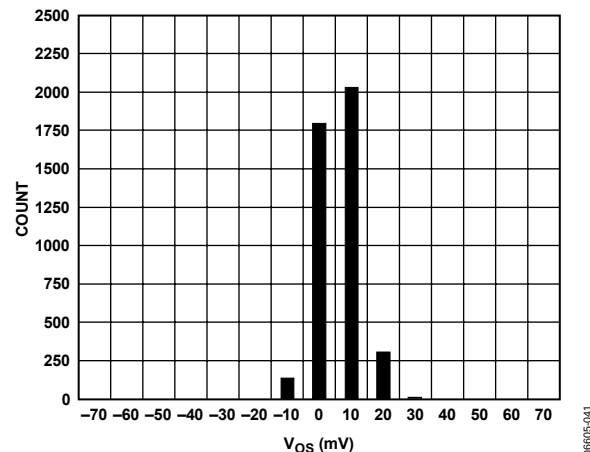
Figure 41. Vos Distribution
