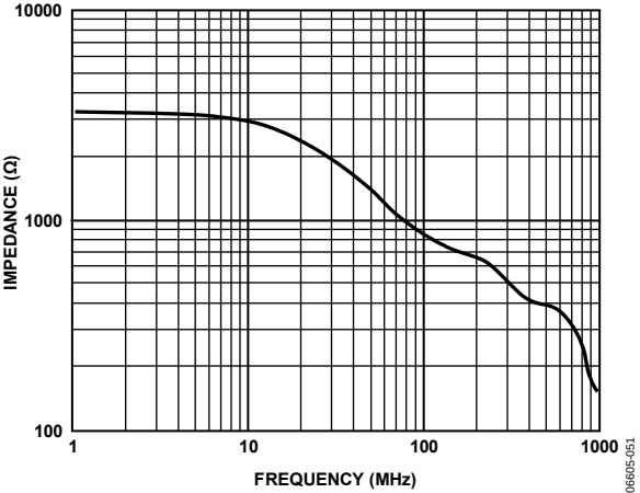
Figure 35. Input Impedance
