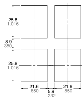
Chassis cutout (Side-by-side installation)
