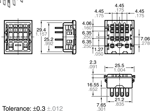
With a relay mounted (HC2-SS-K-H105)
