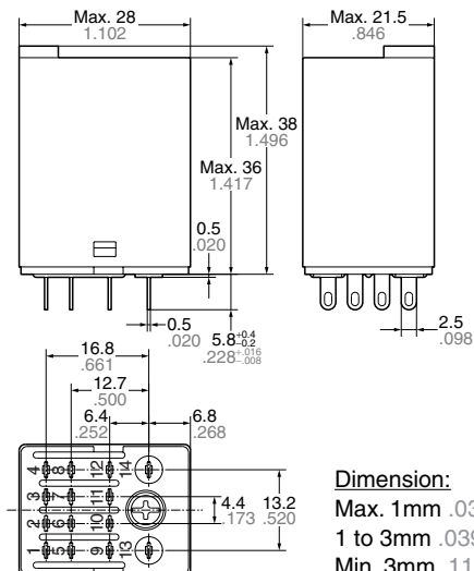
External dimensions
