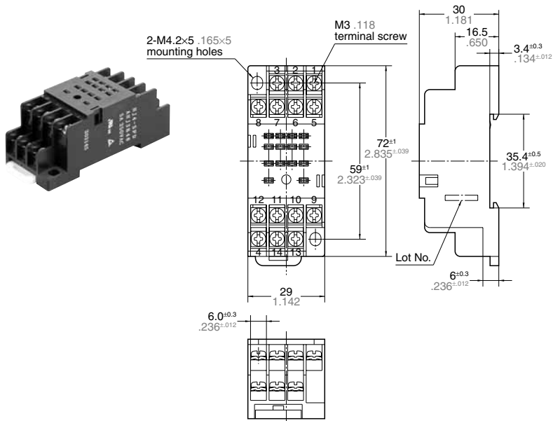
External dimensions
