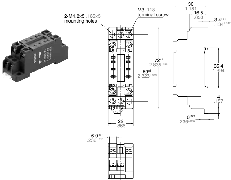
External dimensions
