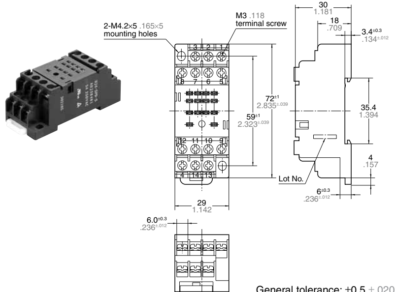
External dimensions
