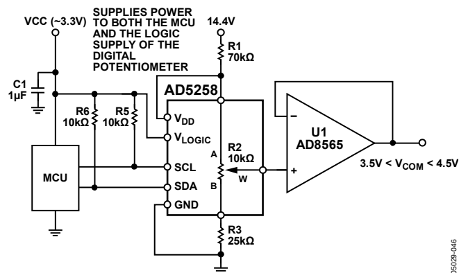
Figure 45. Circuitry When a Separate Supply Is Not Available for V_{\text{DD}}
