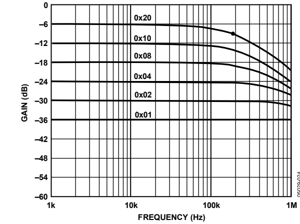
Figure 23. Gain vs. Frequency vs. Code, R_{AB} = 50\text{ k}\Omega
