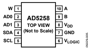
Figure 4. Pin Configuration
