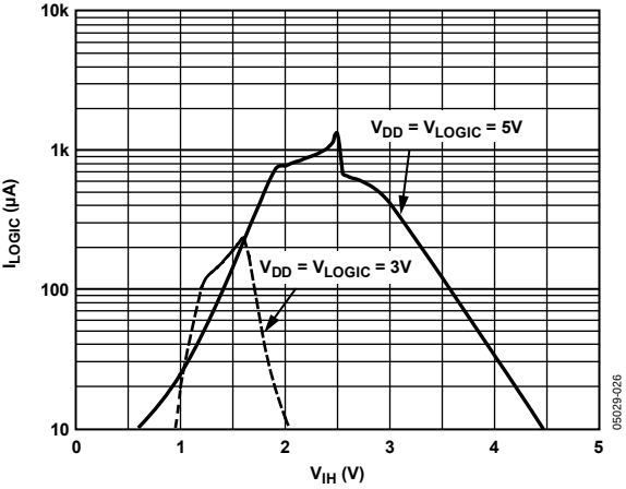
Figure 25. Logic Supply Current vs. Input Voltage
