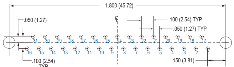
31 PIN M83513/22-E
