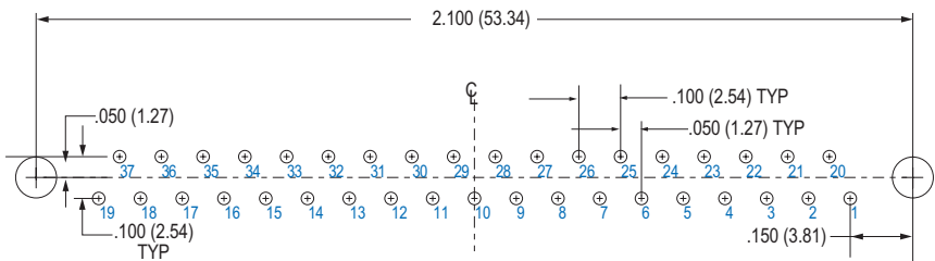
37 PIN M83513/22-F
