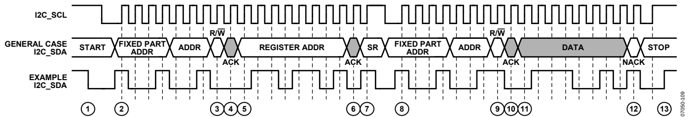
Figure 29. I²C Read Procedure
