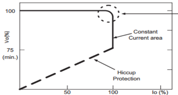
Typical LED power supply I-V curve
