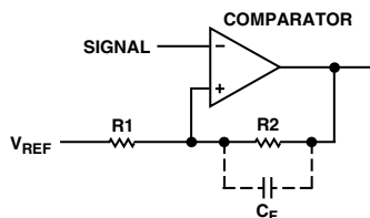
Figure 14. Configuring the AD8564 with Hysteresis
