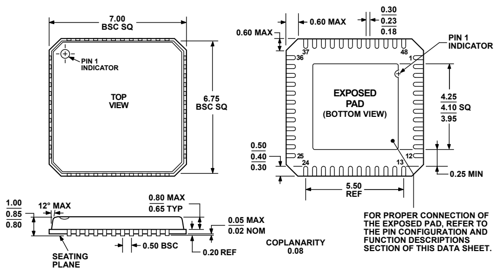
Figure 59. 48-Lead Lead Frame Chip Scale Package [LFCSP_VQ] 7 mm × 7 mm Body, Very Thin Quad (CP-48-3) Dimensions shown in millimeters
