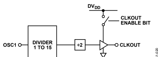
Figure 20. CLKOUT Stage
