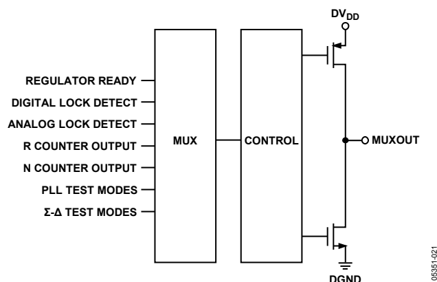
Figure 21. MUXOUT Circuit
