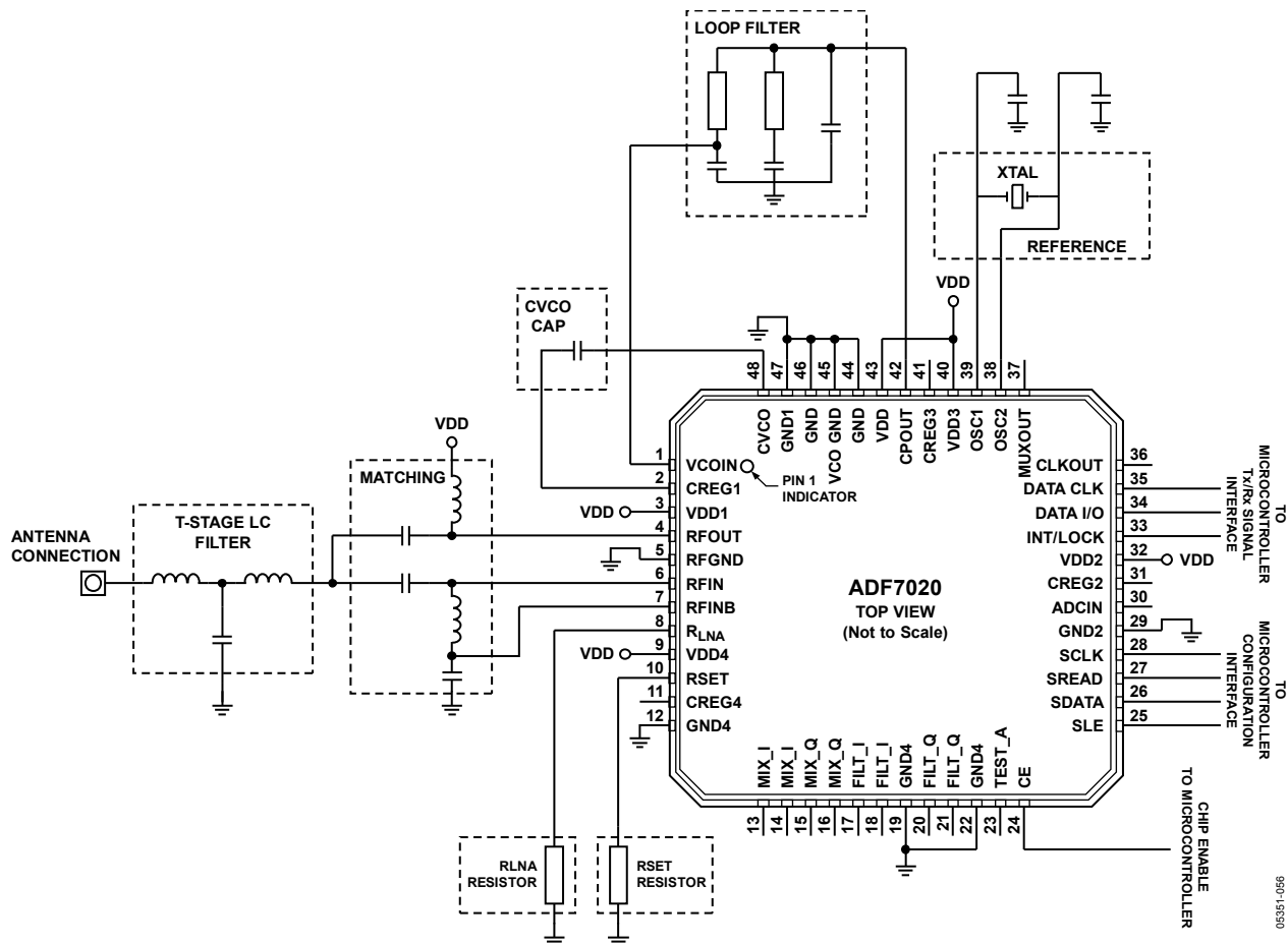
Figure 41. Application Circuit
