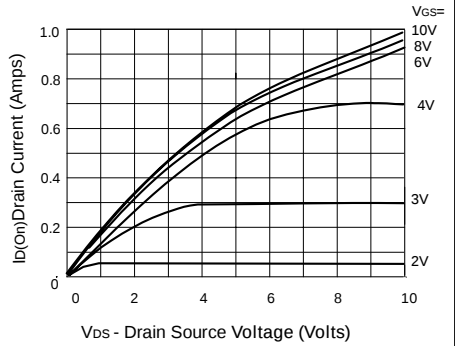
Saturation Characteristics
