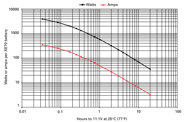
Figure A-20: XE70 discharge data to 11.1V at 25°C (77°F)
