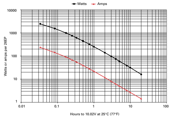
Figure B-10: 26EP discharge data to 10.02V at 25°C (77°F)
