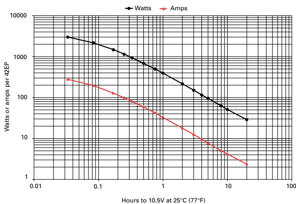
Figure B-15: 42EP discharge data to 10.5V at 25°C (77°F)
