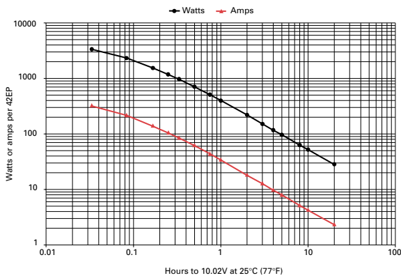
Figure B-14: 42EP discharge data to 10.02V at 25°C (77°F)
