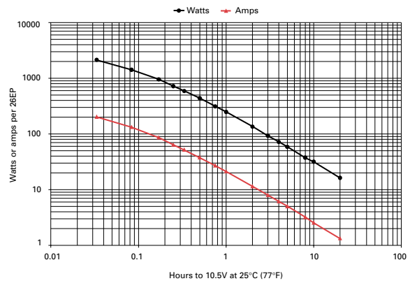
Figure B-11: 26EP discharge data to 10.5V at 25°C (77°F)
