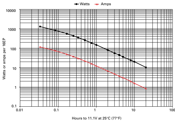
Figure B-8: 16EP discharge data to 11.1V at 25°C (77°F)
