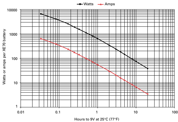
Figure A-17: XE70 discharge data to 9V at 25°C (77°F)
