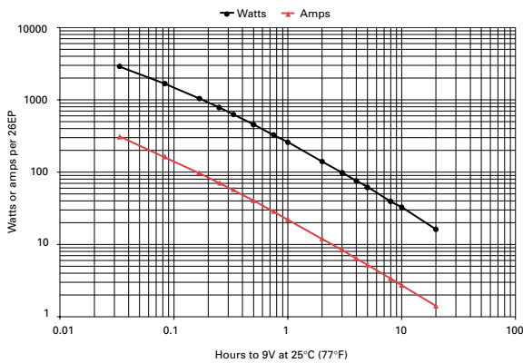
Figure B-9: 26EP discharge data to 9V at 25°C (77°F)
