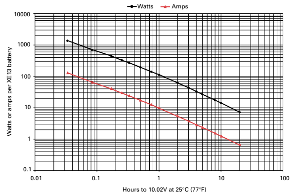
Figure A-2: XE13 discharge data to 10.02V at 25°C (77°F)
