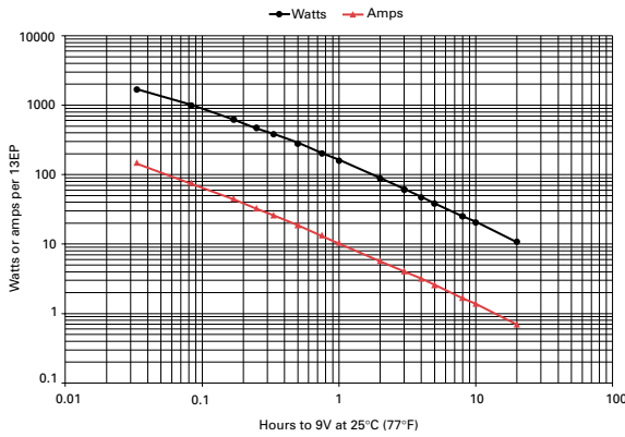
Figure B-1: 13EP discharge data to 9V at 25°C (77°F)
