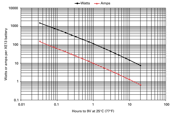
Figure A-1: XE13 discharge data to 9.0V at 25°C (77°F)
