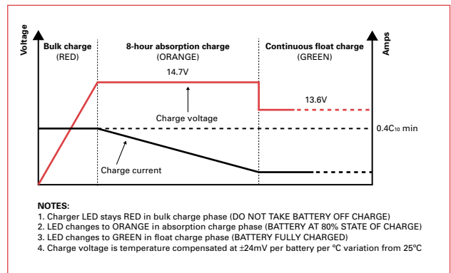
Figure 2.8.1: Three-step (IUU) charge profile
