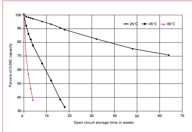
Figure 2.11.2: Storage capacity at temperatures
