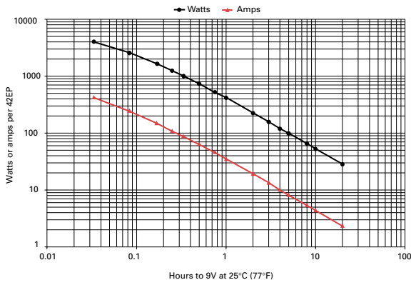
Figure B-13: 42EP discharge data to 9V at 25°C (77°F)
