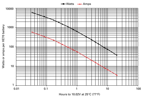
Figure A-18: XE70 discharge data to 10.02V at 25°C (77°F)
