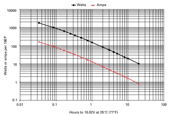
Figure B-6: 16EP discharge data to 10.02V at 25°C (77°F)
