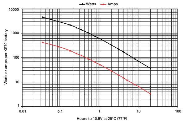
Figure A-19: XE70 discharge data to 10.5V at 25°C (77°F)
