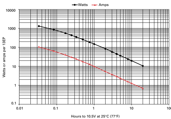
Figure B-3: 13EP discharge data to 10.5V at 25°C (77°F)
