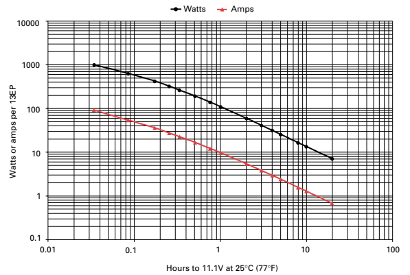
Figure B-4: 13EP discharge data to 11.1V at 25°C (77°F)
