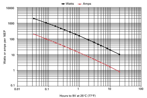
Figure B-5: 16EP discharge data to 9V at 25°C (77°F)
