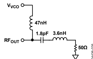
Figure 22. Optimum ADF4360-2 Output Stage
