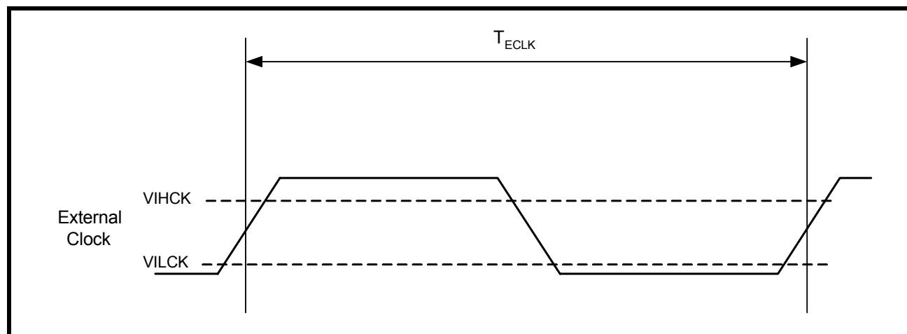
FIGURE 20. CLOCK TIMING
