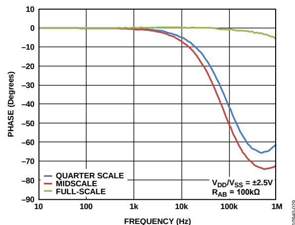
Figure 25. Normalized Phase Flatness vs. Frequency, R_{AB} = 100\text{ k}\Omega
