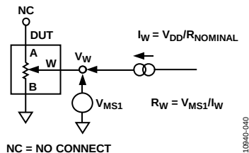
Figure 36. Wiper Resistance
