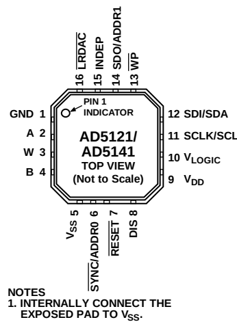
Figure 7. Pin Configuration
