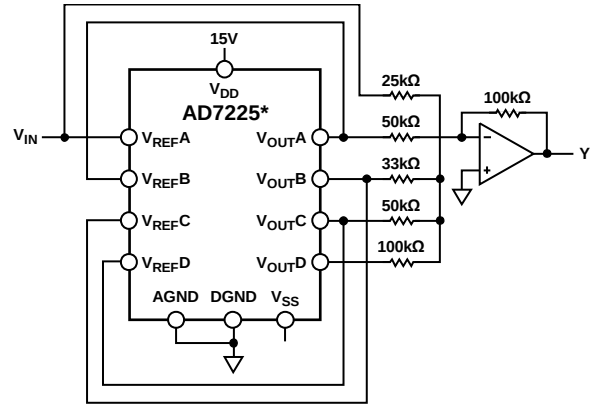
Figure 24. Complex Waveform Generation
