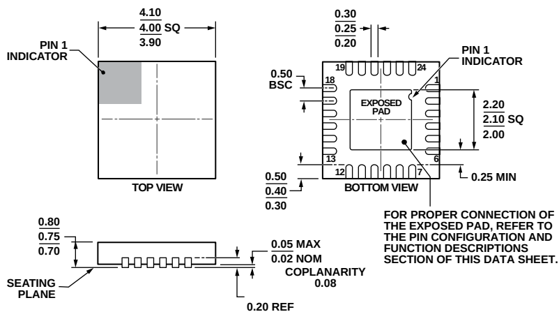
Figure 19. 24-Lead Lead Frame Chip Scale Package [LFCSP_WQ] 4 mm × 4 mm Body, Very Very Thin Quad
