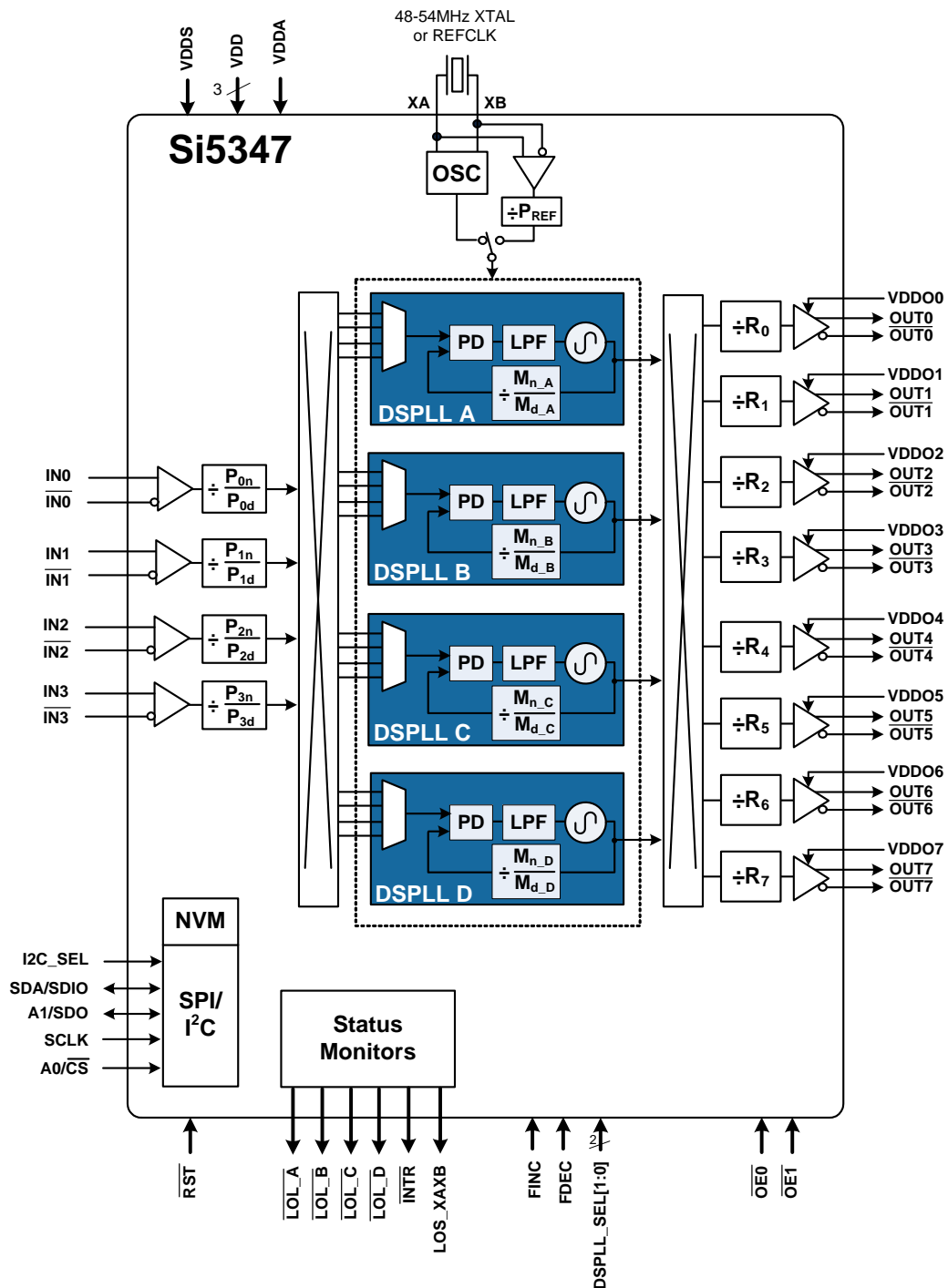
Figure 9. Si5347 Detailed Block Diagram
