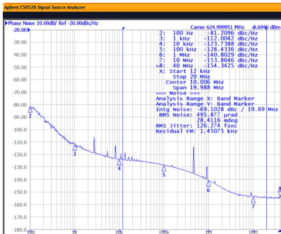
Figure 6. Input = 25 MHz; Output = 625 MHz, 2.5 V LVDS
