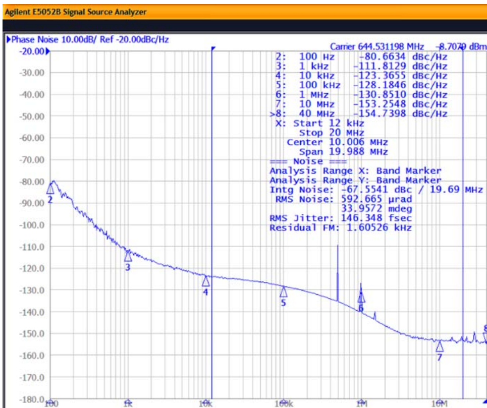
Figure 8. Input = 25 MHz; Output = 644.5311 MHz, 2.5 V LVDS
