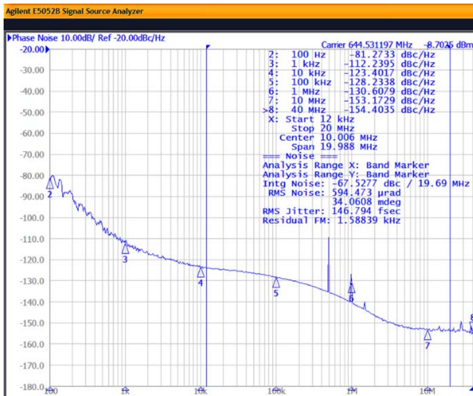
Figure 7. Input = 19.44 MHz; Output = 644.5311 MHz, 2.5 V LVDS
