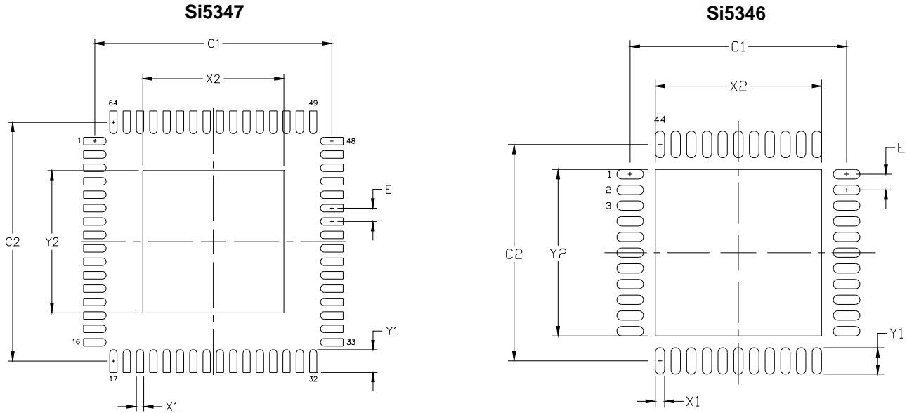
Figure 31. PCB Land Pattern
