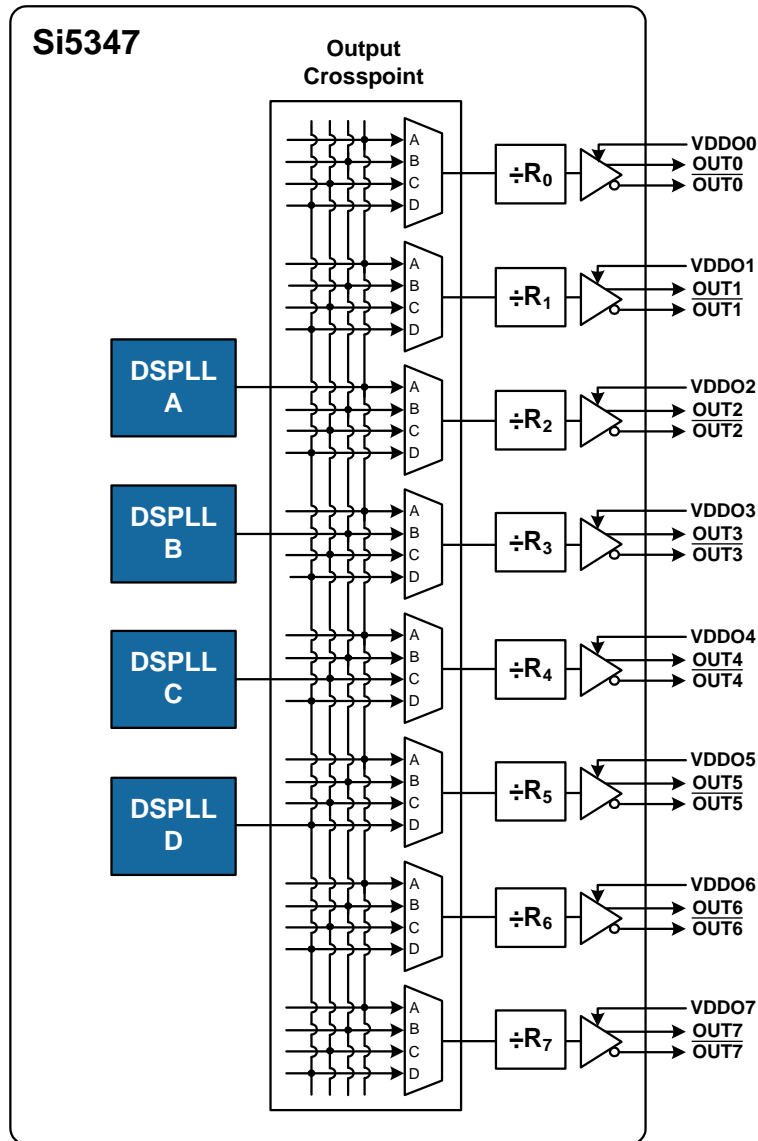
Figure 24. DSPLL to Output Driver Crosspoint
