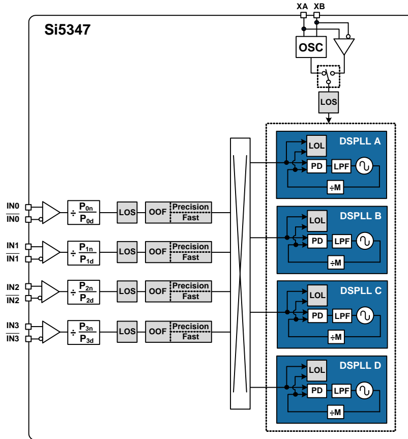
Figure 17. Si5347/46 Fault Monitors
