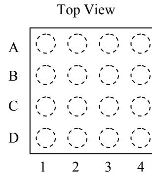
CSBGA (4mm x 4mm)
