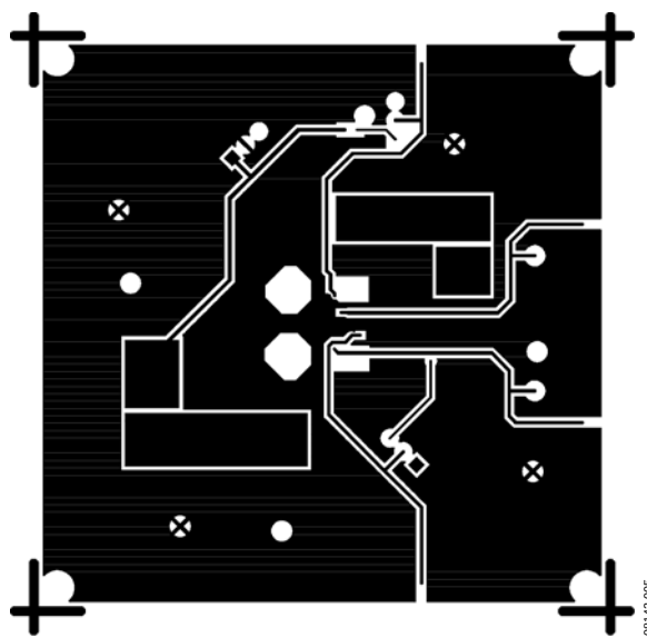
Figure 6. Board Layout Pattern, Circuit Side
