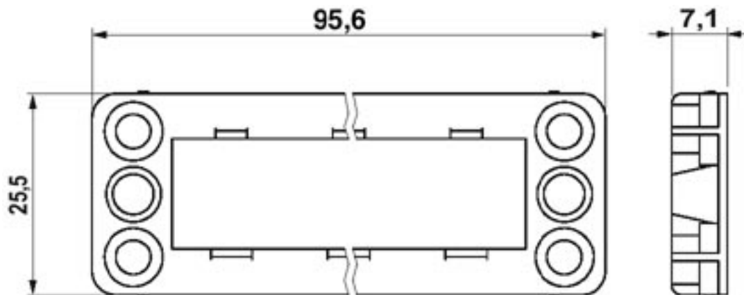
Dimensioned drawing
