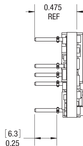
END VIEW
