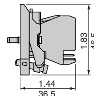
Bodies for pilot lights, plug-in connector Protected LED ZB4BV••4
