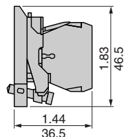
Heads for illuminated push buttons, momentary, for light source LED
