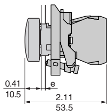
Illuminated push buttons Protected LED XB4BW3••5
