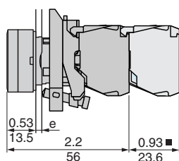
Double headed push buttons with pilot light Protected LED XB4BW84•5
