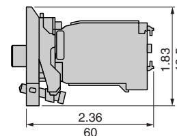
Transformer type, for BA 9s bulb ZB4BV•, BV•D•
