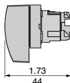
Key switches ZB4BG•, BG0•
