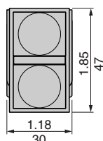
Double headed push buttons with pilot light Protected LED XB4BW84•5
