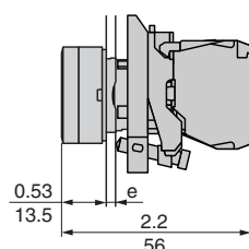
Double headed push buttons with pilot light Protected LED XB4BW84•5
