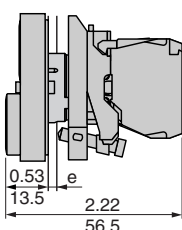
Double headed push buttons with pilot light Protected LED XB4BW84•5
