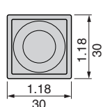
Heads for double-headed push buttons, momentary
