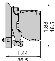
Heads for pilot lights, with light module Protected LED ZB4BV0•3
