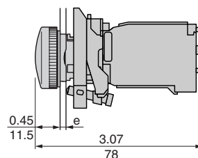
Transformer type XB4BV3•, BV4•
