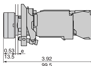
Illuminated selector switches Protected LED XB4BK12••5
