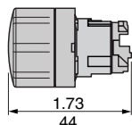
Bodies for push buttons and switches Screw clamp terminal connections ZB4BZ10•, BZ141
