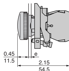
Direct supply XB4BV6
