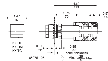
Dual Lamp Push Button Operator
