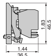
Plug-in connector ZB4BZ10•4, BZ1414
