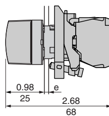
Illuminated selector switches Protected LED XB4BK12••5
