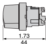
Knurled knob ZB4BD•9
