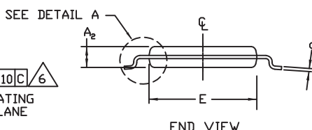
END VIEW
