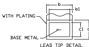
LEAD TIP DETAIL
