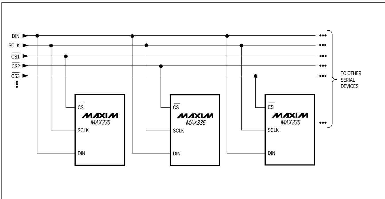
Figure 6. Addressable Serial Interface
