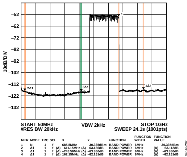
Figure 141. Mid Band Wideband ACLR
