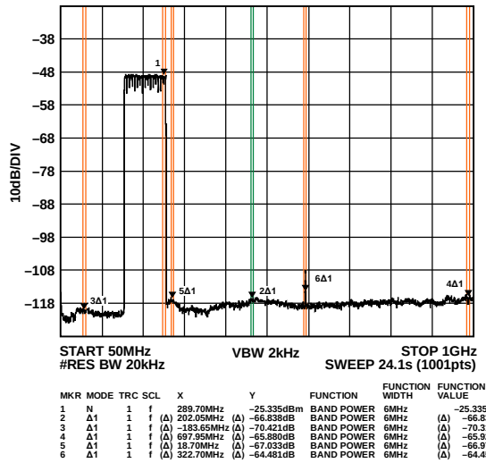
Figure 134. Low Band Wideband ACLR
