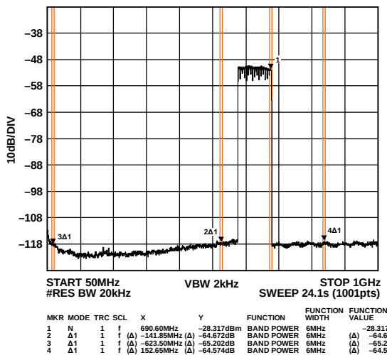
Figure 135. Mid Band Wideband ACLR
