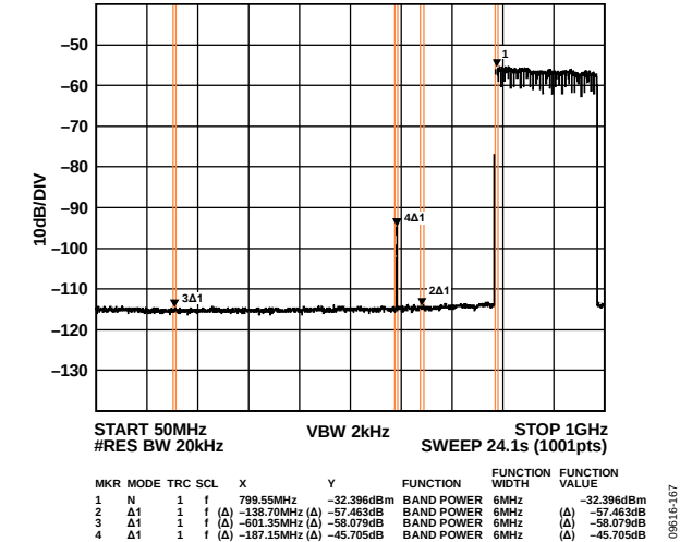
Figure 68. High Band Wideband ACLR
