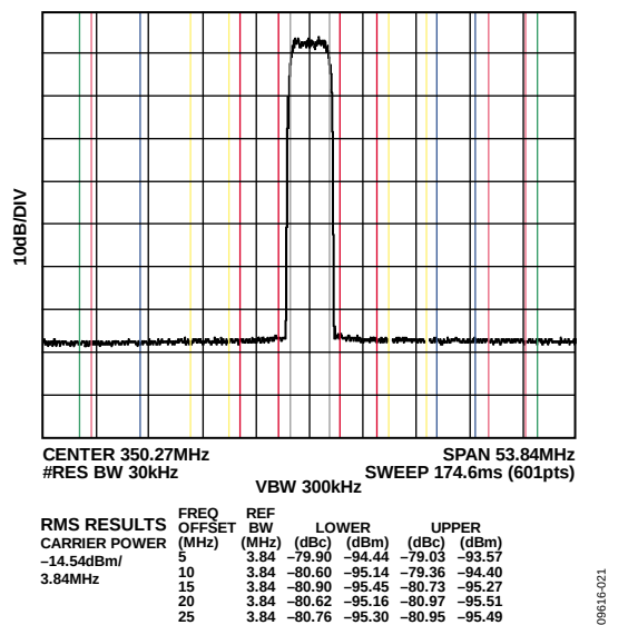
Figure 103. Single-Carrier WCDMA at 350 MHz, f_{DAC} = 2457.6 MSPS
