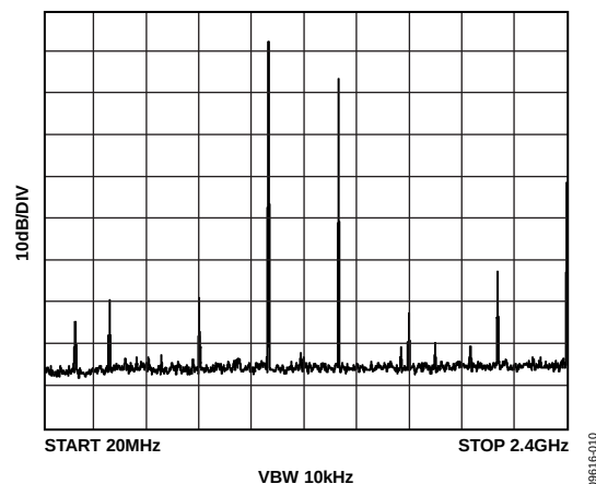
Figure 92. Single-Tone Spectrum at f_{OUT} = 1091 MHz, f_{DAC} = 2.4 GSPS
