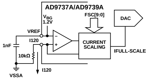
Figure 177. Voltage Reference Circuit
