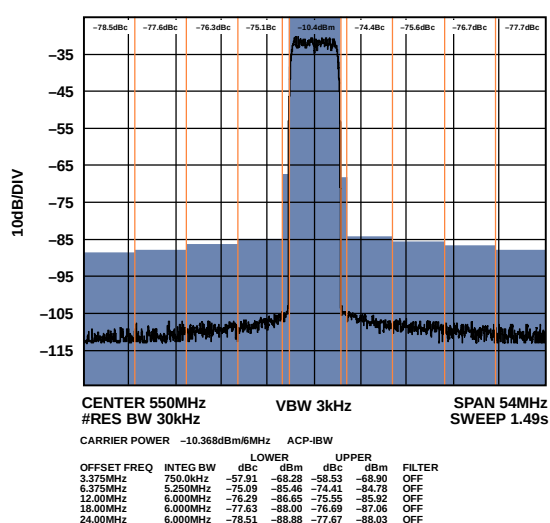
Figure 120. Mid Band Narrow-Band ACLR
