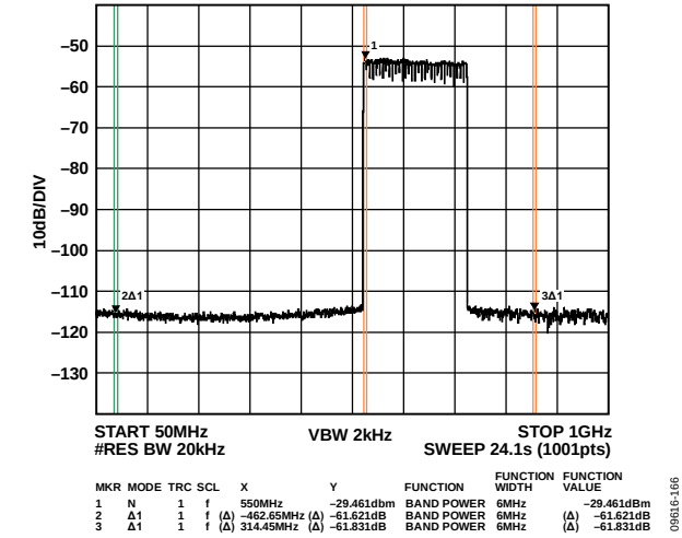
Figure 67. Mid Band Wideband ACLR
