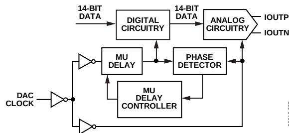
Figure 165. AD9737A Mu Delay Controller Block Diagram
