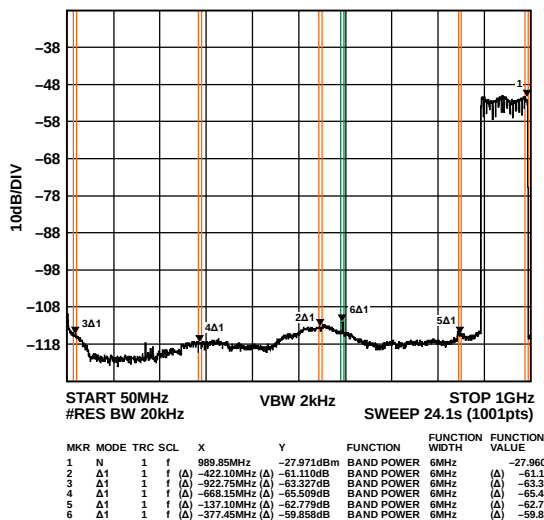
Figure 136. High Band Wideband ACLR
