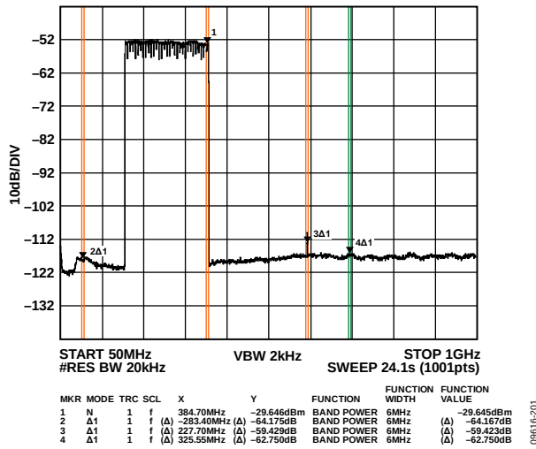
Figure 140. Low Band Wideband ACLR
