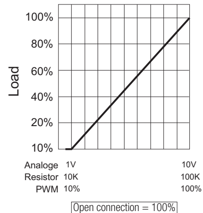
Dimming Curve
