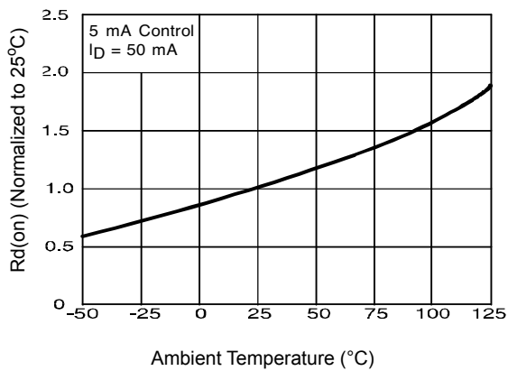
Figure 4. Typical On-Resistance
