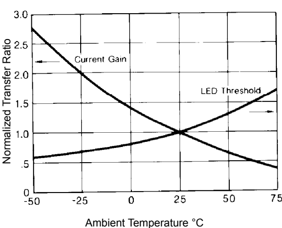
Figure 9. Typical Control Threshold and Transfer Ratio
